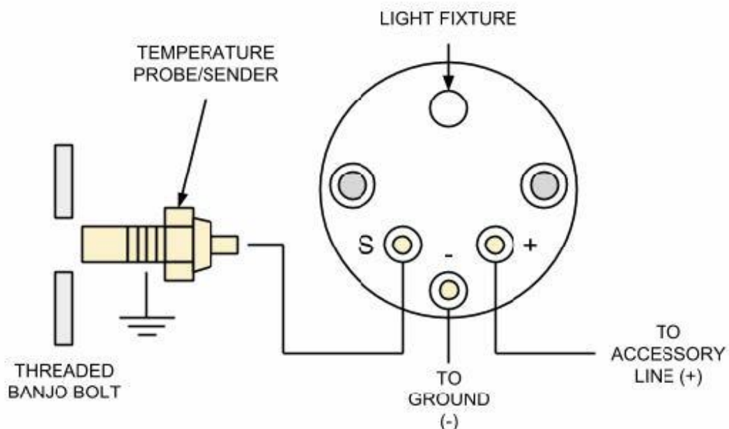
Figure 8.1: Water temperature gauge circuit, (terminals may vary depending on model). Temperature sender grounds to threaded banjo bolt.
